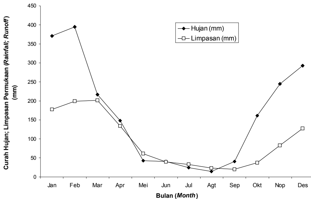
Gambar (Figure) 2. Sebaran data hujan dan limpasan bulanan rata-rata di DPS Kali Sanen ( Distribution of the average monthly rainfall-runoff in Kali Sanen catchment )
